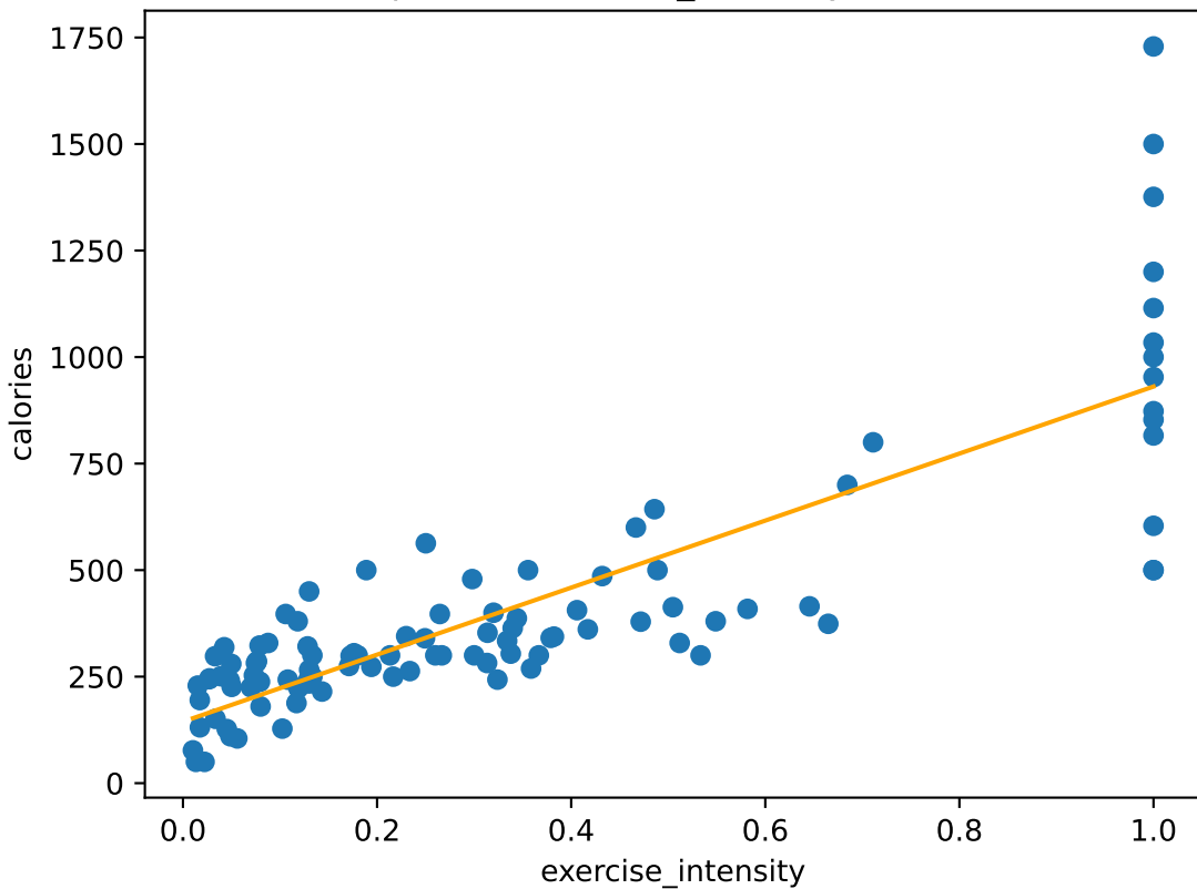
Pairplot for exercise_intensity - calories
